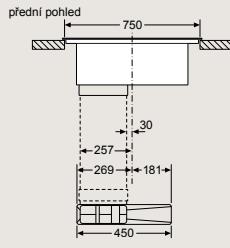
EX870NX68E, EX877NX68E, ED877HQ26E
